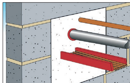
Firewise compound trowled into wall
